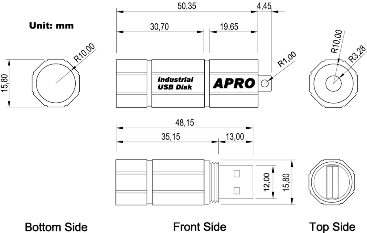
Figure 1: APRO Rugged Metal USB Flash Disk Generation 4 Dimension
